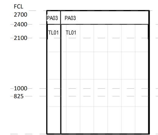
10 ELEVATION DETAIL 1 : 50
