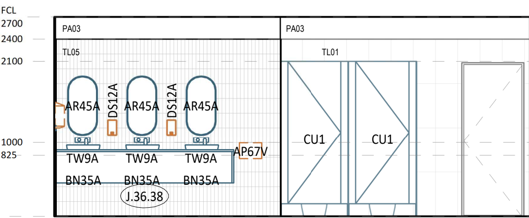
5 ELEVATION DETAIL 1 : 50
