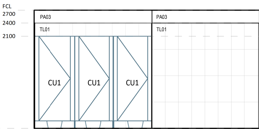
8 ELEVATION DETAIL 1 : 50
