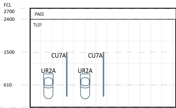
3 ELEVATION DETAIL 1 : 50
