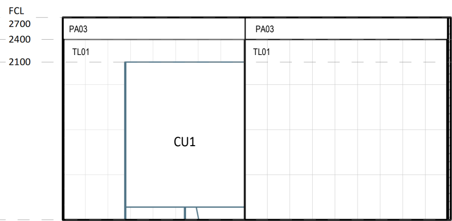
6 ELEVATION DETAIL 1 : 50
