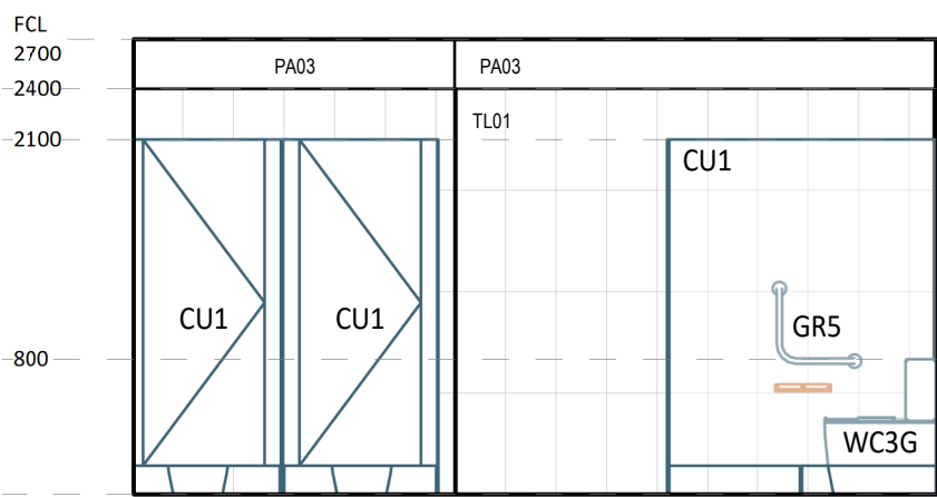
7 ELEVATION DETAIL 1 : 50
