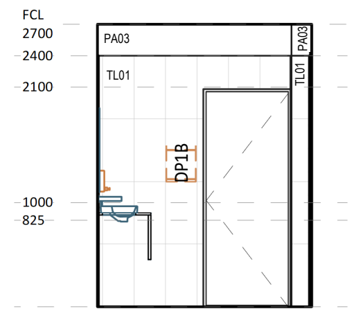
13 ELEVATION DETAIL 1 : 50
