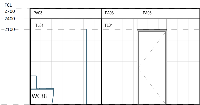
9 ELEVATION DETAIL 1 : 50
