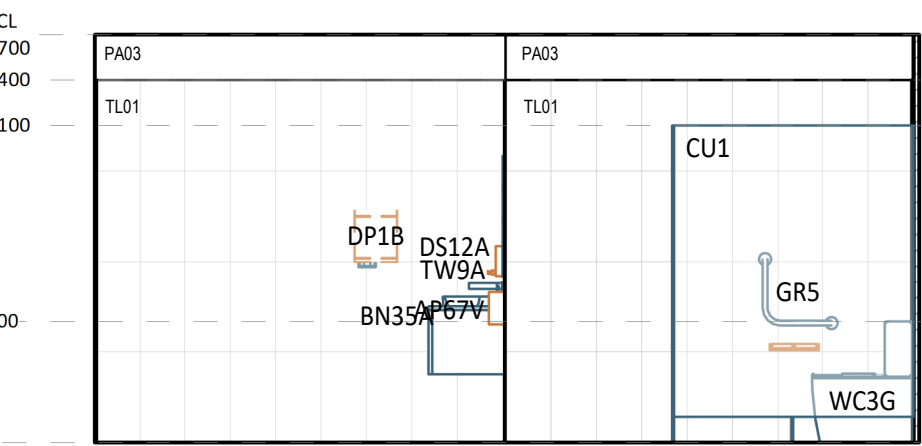
4 ELEVATION DETAIL 1 : 50
