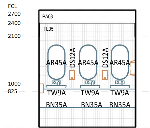
12 ELEVATION DETAIL 1 : 50
