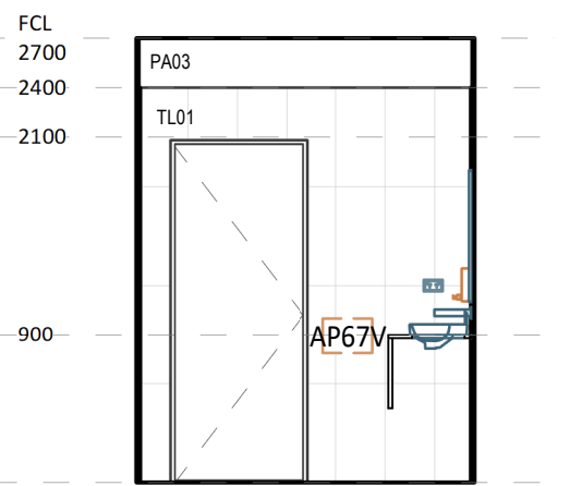
11 ELEVATION DETAIL 1 : 50
